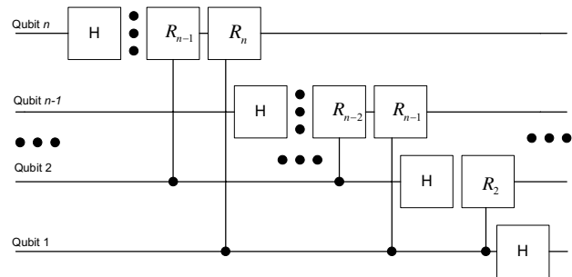
Fig. 9. A N-qubit QFT Circuit
