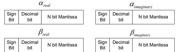
Fig. 2. Fixed-point quantum bit representation
